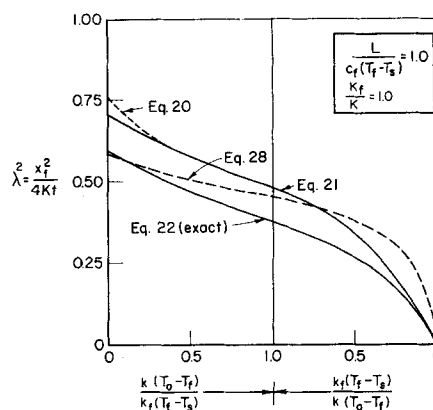
Fig. 9. Effect of k(T_o - T_f)/k_f(T_f - T_s) .
