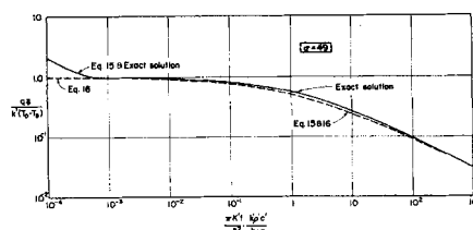
Fig. 7. Comparison of exact and patched solutions for an insulated slab.
