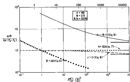
Fig. 4. Bounding solutions for an insulated sphere.
